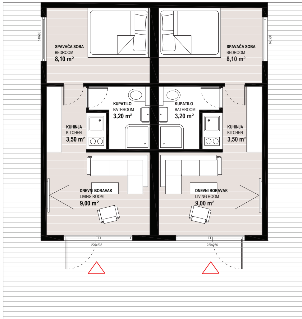
OSNOVA OBJEKTA (GROUND FLOOR)
